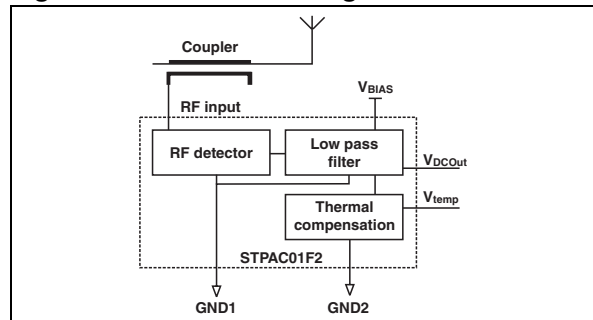
Figure 2. Functional diagram
