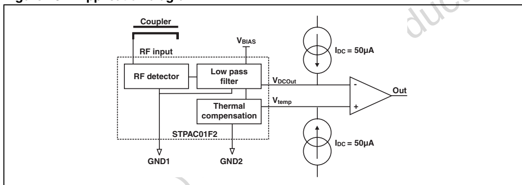
Figure 10. Application diagram
